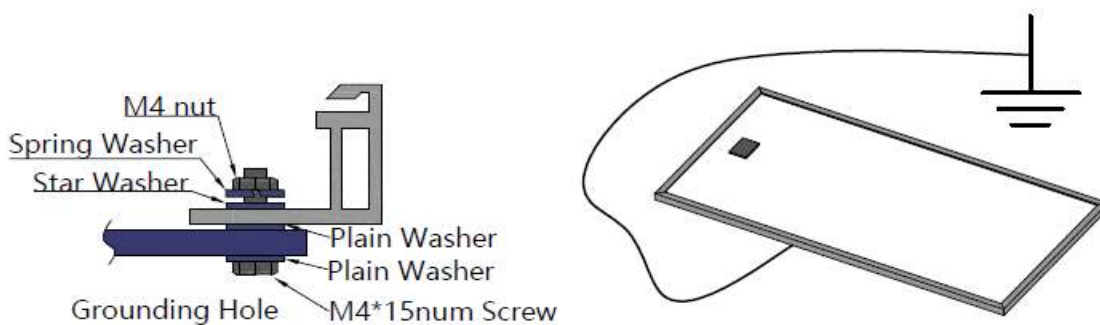
Figure 8: Ground installation of PV modules
