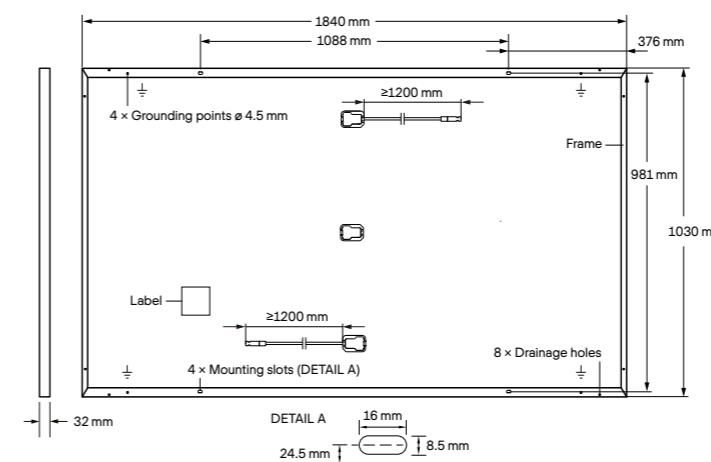
Fig. 1: External dimensions and components for Q.BOOST
